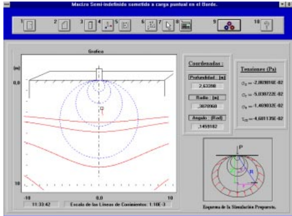
Figure 5. Simulation workplace for a problem in elasticity presents a schematic diagram (esquema) of the problem at the lower right and graph of the computed results (gráfica) at the left. The problem is that of a semi-infinite elastic body subjected to a force at one point on the surface. The buttons are explained in the text.
