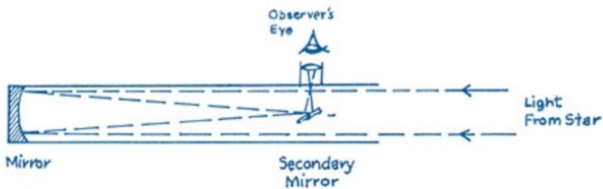
Newtonian Reflector
