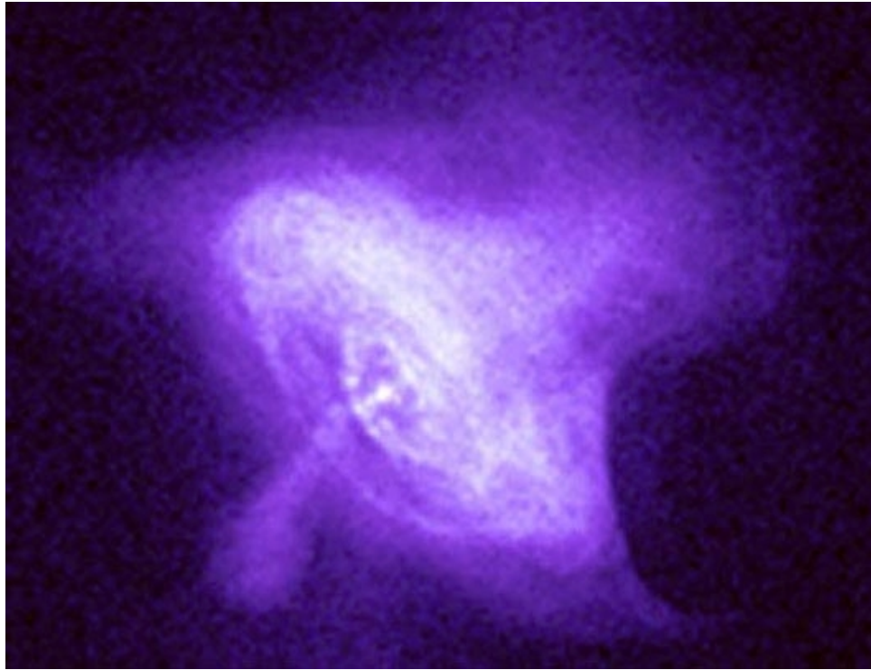
CRAB NEBULA IMAGED IN X-RAYS BY NASA'S CHANDRA OBSERVATORY.
