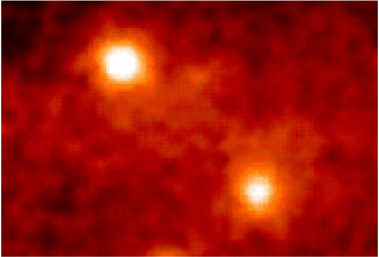
IMAGE OF CRAB NEBULA AND NEARBY REGION AS SEEN IN GAMMA RAY WAVELENGTHS.
