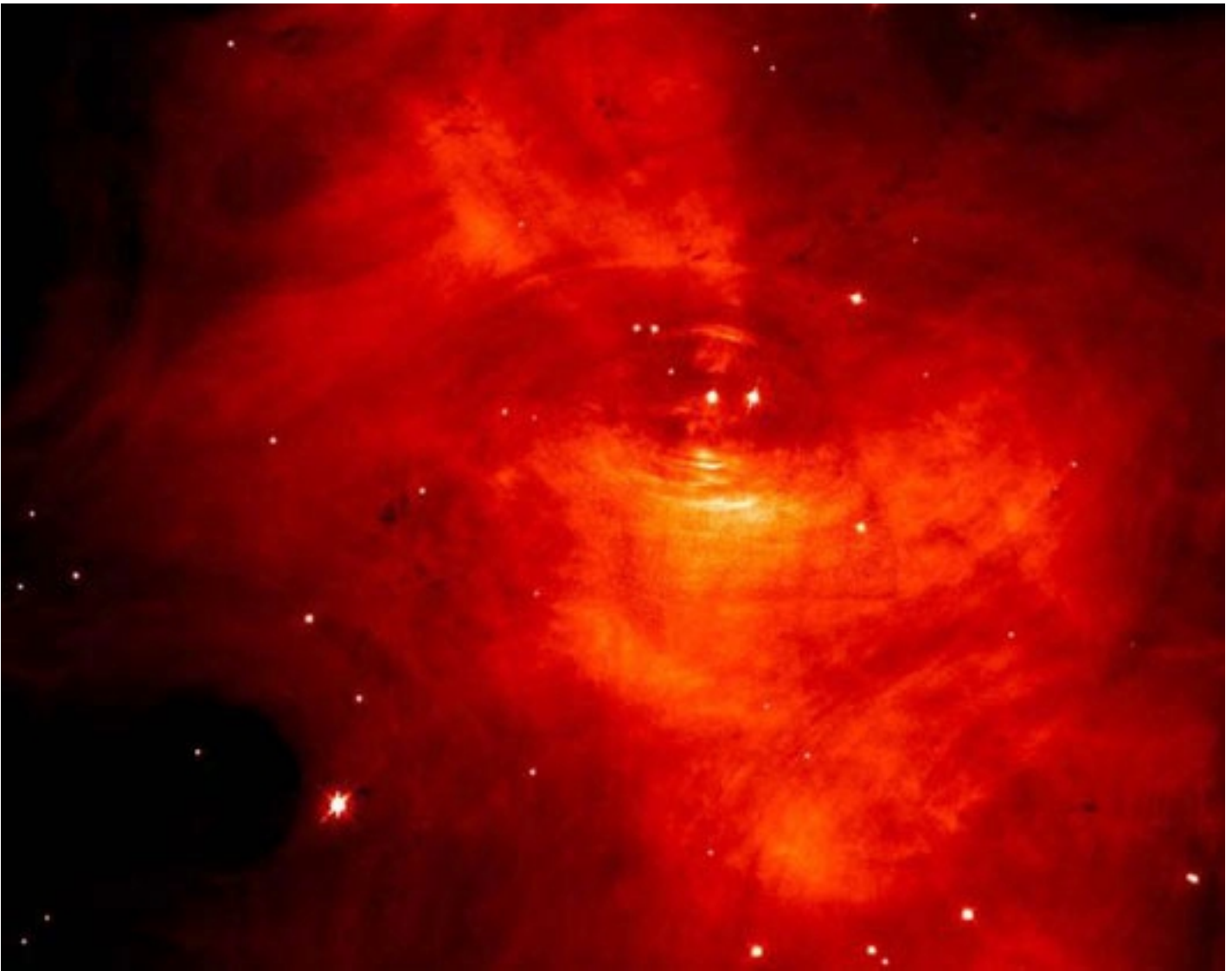
IMAGE TAKEN OF THE CRAB NEBULA IN VISIBLE LIGHT WITH THE HUBBLE SPACE TELESCOPE.
