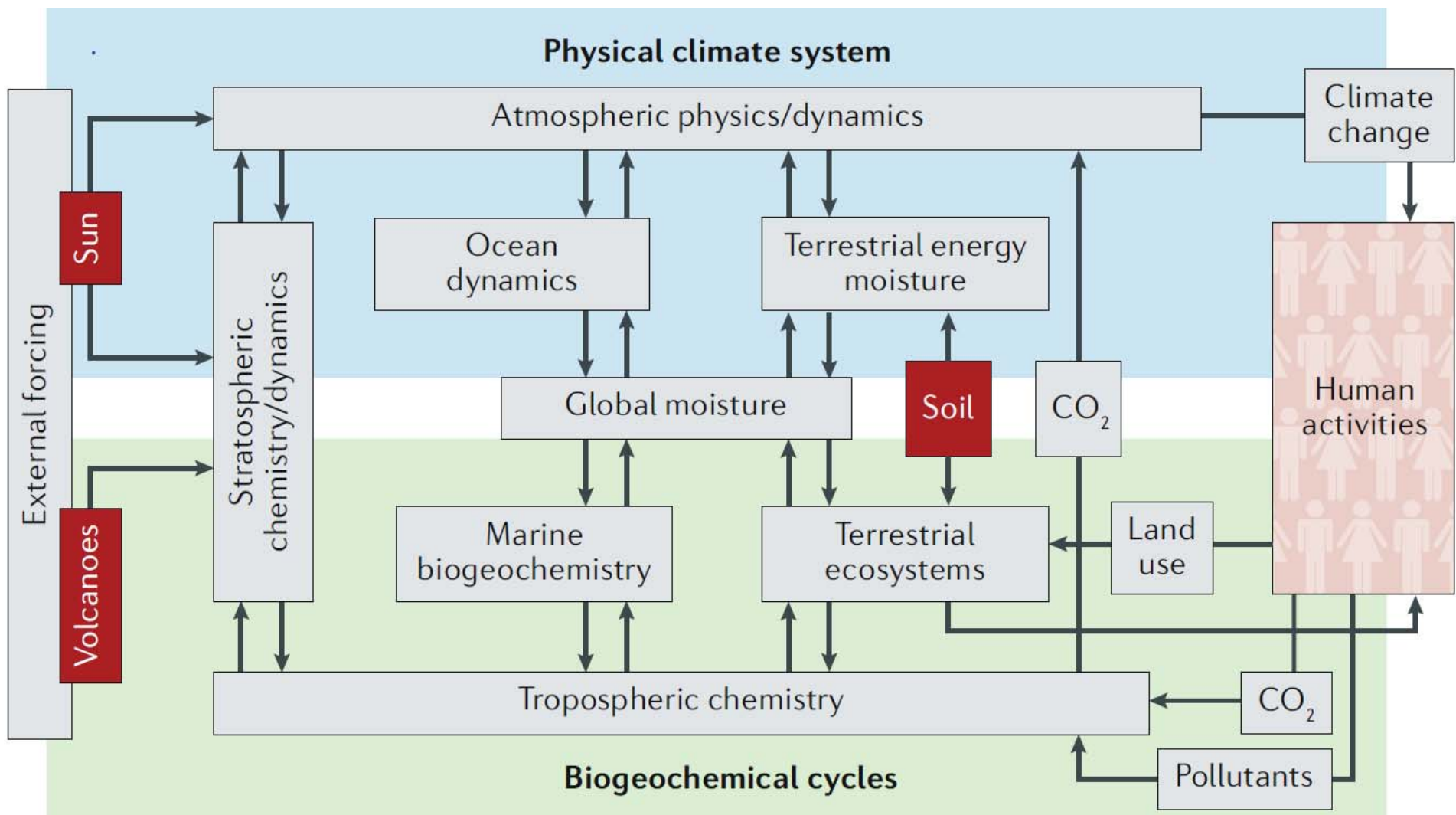
“Bretherton Diagram”
