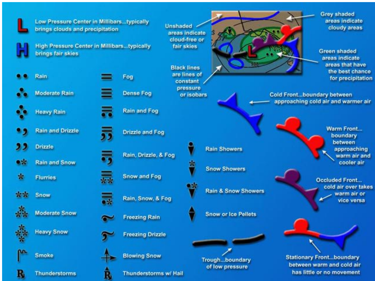
Image from http://weather.about.com/od/forecastingtechniques/ss/mapsymbols_2.htm
